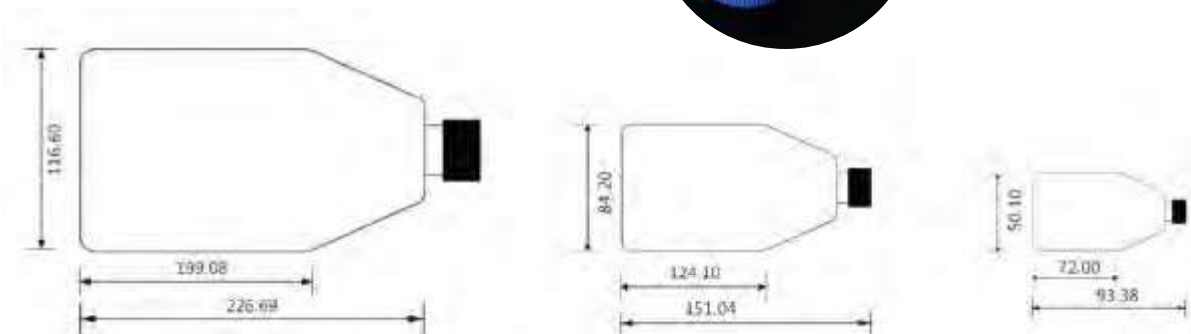
Dimensions = mm
